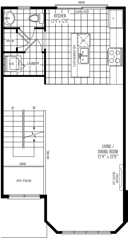
SECOND FLOOR | ELEV. A
