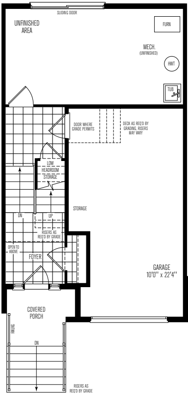
GROUND FLOOR | ELEV. A & B
